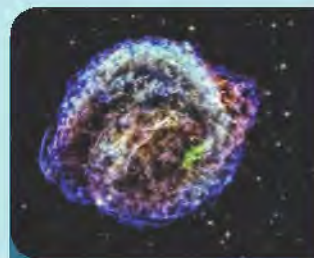
Kepler's Supernova
